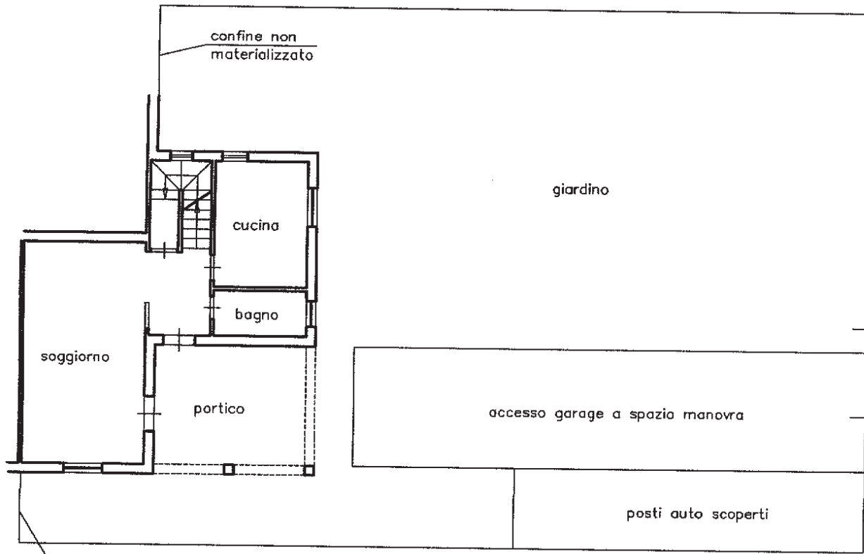
PIANO TERRENO
